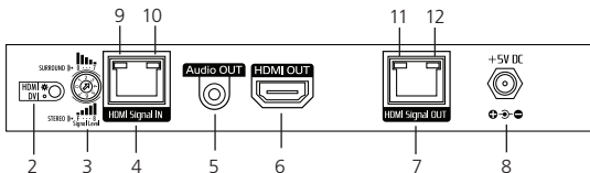
Figure 2-7. Cascadable receiver's back panel.
